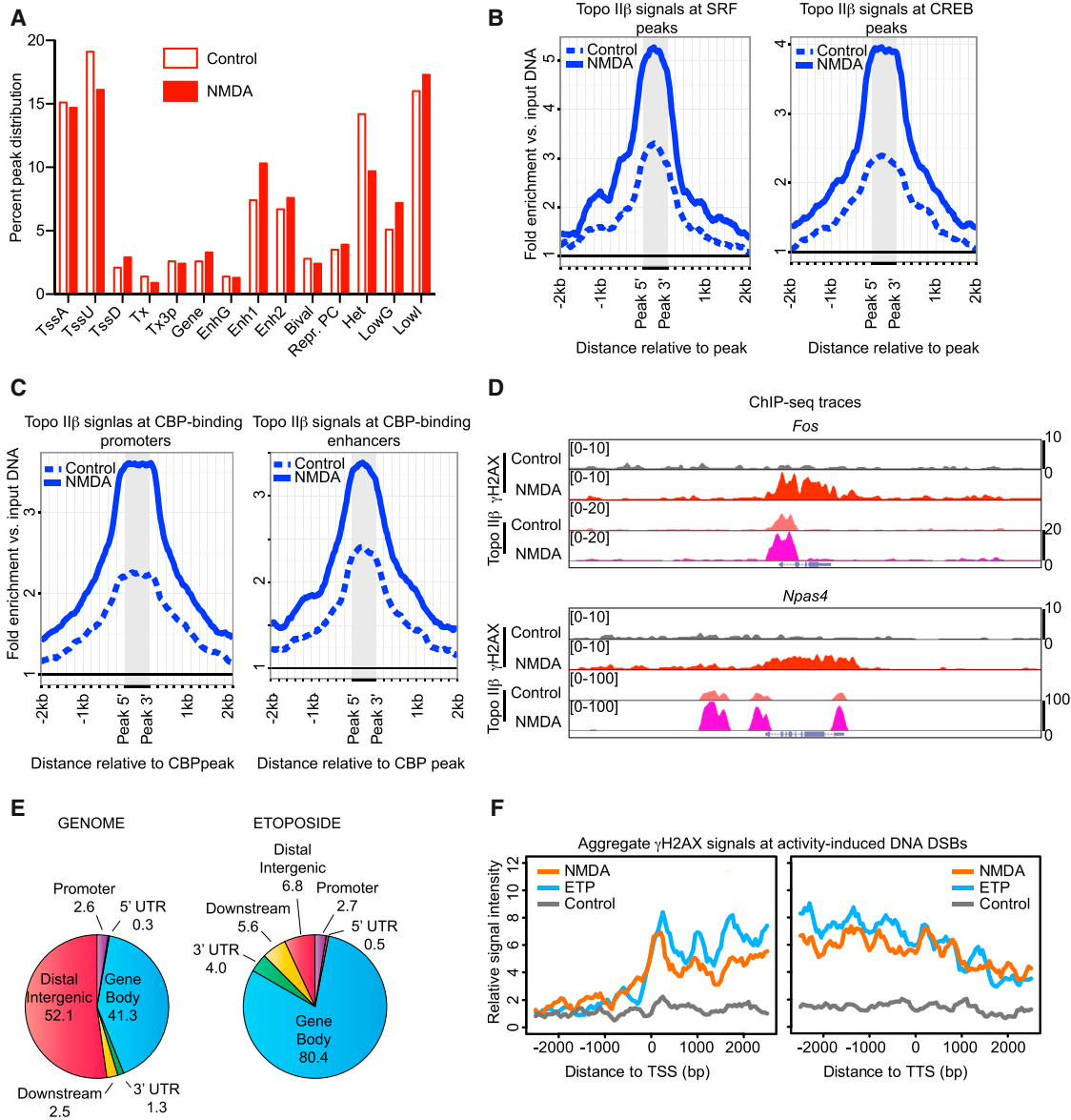
Figure 4. Genome-wide Topo II \beta DNA Cleavage Patterns Coincide with the Sites of Neuronal Activity-Induced DSBs
