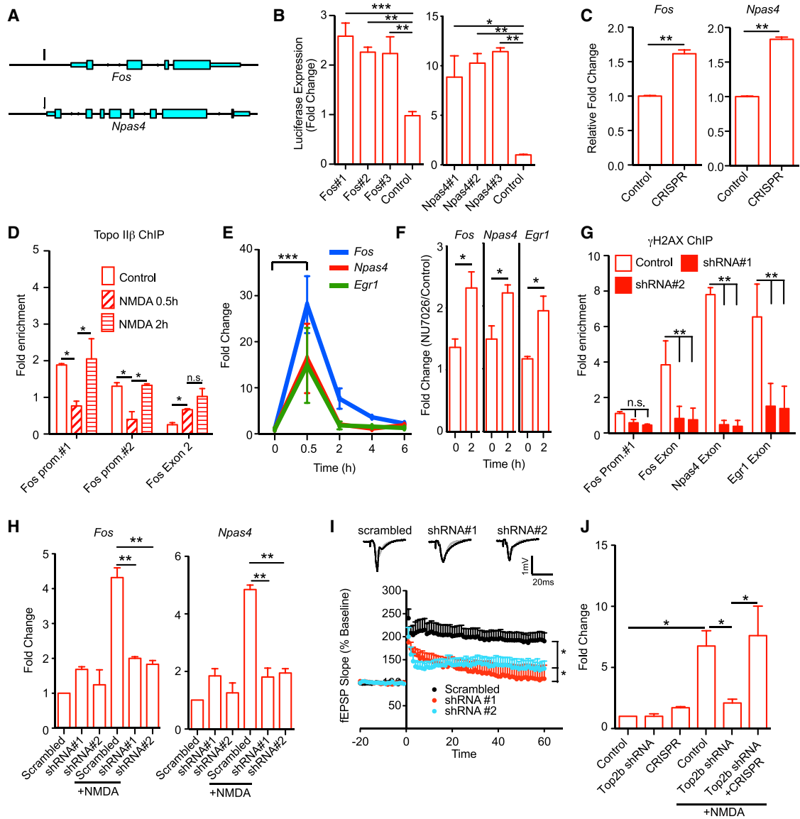
Figure 6. Topo IIβ-Mediated DNA DSBs Govern the Expression of Early-Response Genes Following Neuronal Activity
