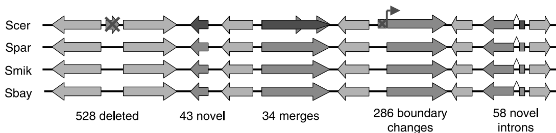
FIG. 11. Revised gene catalogue. Our comparative analysis has revised the yeast gene annotation, affecting nearly 15% of all currently annotated genes. We found that 528 previously annotated ORFs are not real genes, identified 43 novel short ORFs that were previously overlooked, proposed merges of 34 pairs of consecutive ORFs, proposed 286 boundary changes (210 start changes and 76 stop changes), and identified 58 novel introns.
