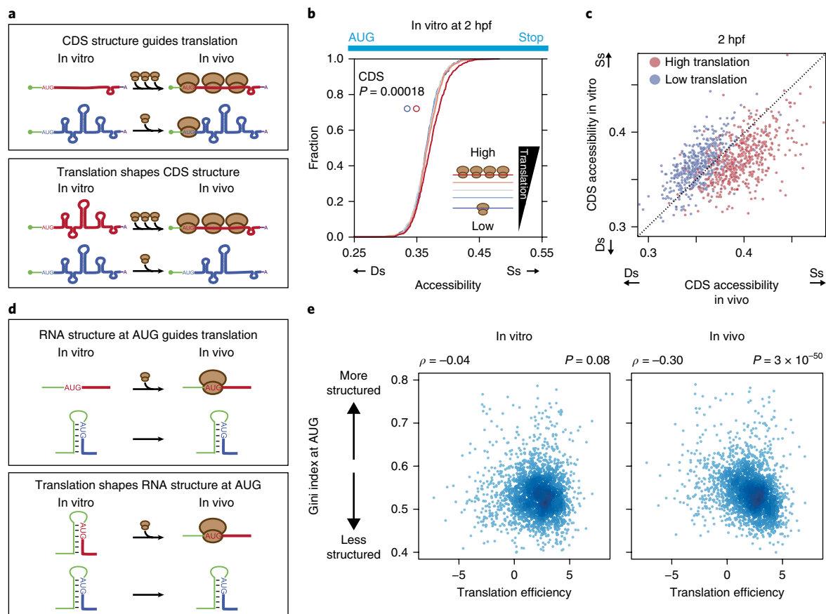
Fig. 2 | Globally, mRNA intrinsic structure is not a main driver of translation. a , Schematic representation of the two models that might explain the observed anticorrelation between translation efficiency and RNA structure in CDS regions in vivo. In the first model, preexisting CDS RNA structures guide translation (top; this is not supported by our analysis). In a second model, translating ribosomes are responsible for the unfolding of CDS RNA structures (bottom; consistent with our analysis). b , Cumulative distributions of global CDS RNA accessibility in vitro at 2 hpf, displaying no difference among mRNAs with different translation efficiency. Transcripts ( n = 2,526 ) were binned into quintiles according to their translation efficiency. P value was computed with a one-sided Mann–Whitney U test. Although P was < 0.05 , we considered this change nonsignificant, given the magnitude of the change and the large sample size; this conclusion is further supported by the scatter-plot analysis in Supplementary Fig. 2c. c , Scatter plot between in vivo and in vitro CDS accessibility at 2 hpf. In vivo, the accessibility was higher for highly translated mRNAs (red dots) and lower for weakly translated mRNAs (blue dots). d , Schematic view of the two models in which RNA structure at the AUG initiation codon is either the cause (top) or the result (bottom) of mRNA translation. e , Correlation between translation efficiency and the structure at AUG regions ( n = 2,360 ), for both in vitro (left) and in vivo (right) conditions. Spearman correlation coefficients ( \rho ) and the corresponding asymptotic P values are shown.
