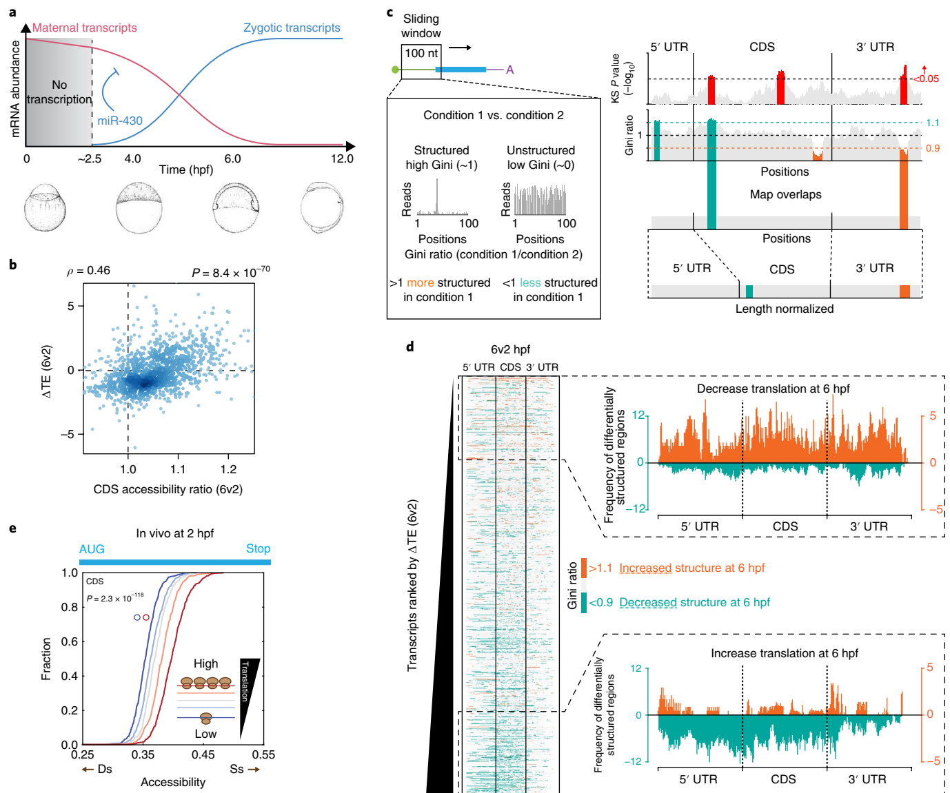
Fig. 1 | Relationship between mRNA structure and translation during the MZT. a , Schematic view of the transcriptomic remodeling that occurs during the MZT. After a transcriptionally silent period (gray), the maternal program (pink) transitions to a zygotic program (blue). b , Correlation between the per-transcript changes at 6 hpf versus 2 hpf (6v2) in translation efficiency ( \Delta TE, 6 - 2 hpf) and CDS accessibility (6/2 hpf) for 1,337 coding sequences with high coverage at both stages. The Spearman correlation coefficient ( \rho ) and the corresponding asymptotic P value are shown. c , Methodology used to identify local RNA structure changes between conditions. Differentially structured (DS) sliding windows are defined as those that are significantly changing ( P < 0.05 ) on the basis of the Kolmogorov-Smirnov test, and show an increase ( >1.1 ) or decrease ( <0.9 ) in their Gini-index ratio. d , Left, structure changes of each 100-nt window (Gini ratio 6/2 hpf) along each transcript (total of 1,273). Transcripts are ranked according to their changes in translation efficiency during the MZT (6 - 2 hpf). Each transcript region (5' UTR, CDS and 3' UTR) is normalized to its length. Right, cumulative distributions of differentially structured windows for transcripts with increased (top 20%, top) and decreased (bottom 20%, bottom) translation. e , Cumulative distribution of global CDS accessibility in vivo, showing that highly translated mRNAs exhibit increased CDS accessibility in vivo at 2 hpf, a stage at which the rate of translation spans \sim 10,000 -fold between highly and weakly translated mRNAs. Ss, single-stranded; ds, double-stranded. Transcripts ( n = 2,526 ) were binned into quintiles according to their translation efficiency. P value was computed with a one-sided Mann-Whitney U test.
