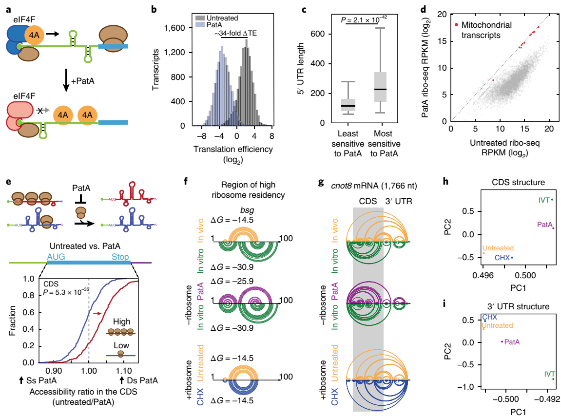
Fig. 3 | Ribosomes promote alternative mRNA structures in the early embryo. a , Schematic view of the PatA translation-inhibition mechanism. PatA decreases the levels of functional eIF4F initiation complex, which is essential for cap-dependent translation, by trapping eIF4A (4A) on mRNAs and ectopically enhancing its RNA helicase activity. b , Distribution of translation efficiencies of PatA-treated (blue) and untreated (gray) embryos. c , Correlation between 5'-UTR length and sensitivity to PatA treatment. The mRNA subgroups least and most sensitive to PatA correspond to the top ( n=394 transcripts) and bottom ( n=394 transcripts) quintiles of the change in translation efficiency (PatA - untreated), respectively. P value was computed with a one-sided Mann-Whitney U test. Box, first to last quartiles; whiskers, 1.5 \times interquartile range; center line, median. d , Scatter plot of the per-transcript ribosome footprints (ribo-seq ribosome profiling) in PatA-treated versus untreated embryos. Results for mitochondrial genes (red), which were unaffected by PatA treatment, remained unchanged. RPKM, reads per kilobase per million reads. e , Schematic representation depicting the effect of PatA, along with its corresponding cumulative distribution of CDS accessibility ratios (untreated/PatA). Accessibility (red arrow) was lower in highly translated mRNAs (red, n=392 ) in PatA-treated than untreated embryos, an effect not observed for weakly translated mRNAs (blue, n=392 ). P value was computed with a one-sided Mann-Whitney U test. f , Arc plots of DMS-seq-guided RNA secondary-structure predictions of a high-ribosome-occupancy region found in the bsg ( basigin ) gene. Each arc represents a base-pair interaction. g , Arc plots of DMS-seq-guided RNA secondary-structure predictions of the full-length cnot8 mRNA from SeqFold. The CDS region is shadowed in gray. h,i , Principal component (PC)-analysis biplots of the SeqFold mRNA structure predictions of the four tested conditions (untreated, in vitro, PatA treated and CHX treated) for CDS ( h , n=1,130 ) and 3'-UTR ( i , n=1,085 ) regions. Source data for h and i are available online.
