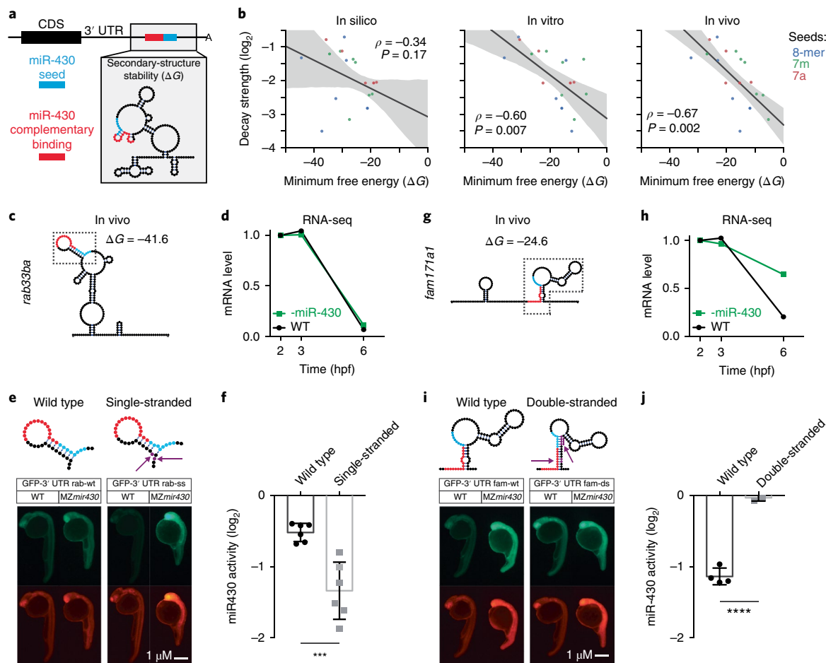
Fig. 6 | Cellular-specific 3'-UTR structures modulate miR-430 activity and gene expression. a , Cartoon representation of the RNA secondary structure found at a miR-430 target site. b , Correlation between the decay strength and the stability of the RNA structure of 18 endogenous miR-430-binding sites (colored according to their seed type), where the RNA secondary structure was predicted with an in silico approach (left) or DMS-seq guided by in vitro (middle) or in vivo structural data (right). Spearman correlation coefficients ( \rho ), asymptotic P values and regression models (shaded region) are shown ( n = 18 different miR-430-binding sites). c, g , In vivo predicted secondary structure and stability ( \Delta G ) of the miR430-target site found in the rab33ba 3' UTR ( c ) and in the fam171a1 3' UTR ( g ). d, h , Changes in mRNA abundance during the MZT of the endogenous rab33ba ( d ) and fam171a1 ( h ) transcripts in wild-type (WT) conditions (black, average of two independent RNA-seq replicates) or in conditions in which miR-430 activity is inhibited (green, one RNA-seq replicate). e, i , Fluorescence microscopy at 24 hpf of GFP reporters containing either a wild-type sequence of the rab33ba ( rab-wt ) or fam171a1 ( fam-wt ) target site, compared with a destabilized version of rab33ba ( rab33ba single-stranded, rab-ss ( e )) or a stabilized version of fam171a1 ( fam171a1 double-stranded, fam-ds ( i )) target site in the 3' UTR. The specific mutations of the rab-ss and fam-ds constructs are highlighted in purple and with arrows. DsRed mRNA was co-injected as a control. Reporters were injected in both the wild type and the maternal-zygotic mutant of miR-430 (MZmir430) lacking the entire miR-430 locus. f, j , miR-430 activity calculated from the fluorescence of the GFP normalized to DsRed and the GFP/DsRed ratio of the MZmir430 mutants for each construct. Data are represented as mean \pm s.d. ( f : wt, n = 6 ; ss, n = 6 ; j : wt, n = 4 ; ds, n = 3 independent replicates). Student t -test P values (two tailed) are indicated as *** P < 0.001 and **** P < 0.0001 . Source data for b , d , h , f and j are provided online.
