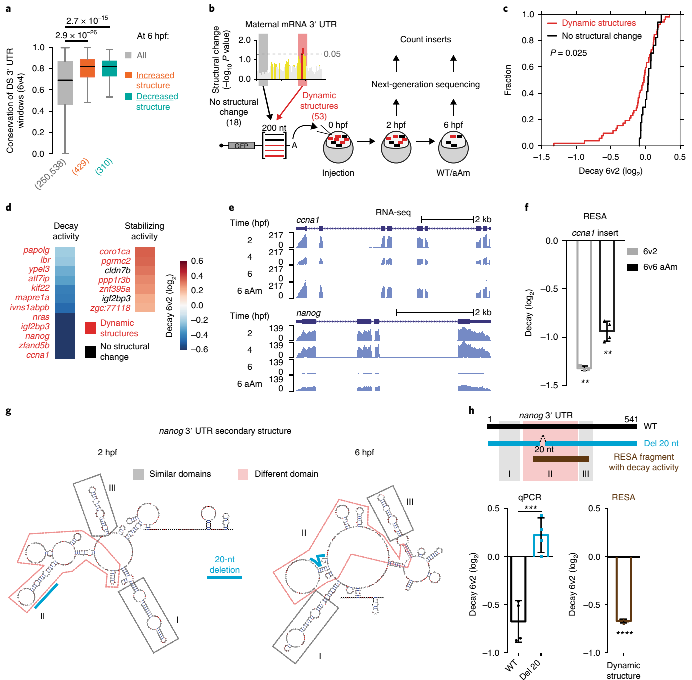
Fig. 7 | Dynamic 3'-UTR structures are enriched in decay regulatory elements. a , Sequence conservation of differentially structured 3'-UTR regions between 4 and 6 hpf (6v4), compared with all 3'-UTR regions analyzed (gray). P values were computed with one-sided Mann-Whitney U tests. Box, first to last quartiles; whiskers, 1.5 \times interquartile range; center line, median. b , Cartoon representation of the RESA experiment used to validate the regulatory activity of 3'-UTR regions that were identified as changing (red) or not changing (gray) in their RNA structure during the MZT. c , Cumulative distribution of the decay activity measured by the RESA validation experiment for 3'-UTR regions with dynamic structures ( n = 53 , red) or with no structural change ( n = 18 , black) during the MZT. P value computed by one-sided Mann-Whitney U test. d , RESA-validated 3'-UTR sequences with identified decay or stabilizing elements. e , Endogenous mRNA expression of ccna1 and nanog at 2, 4 and 6 hpf, as well as for \alpha -amanitin (aAm)-treated embryos collected at 6 hpf. f , Quantification of the decay activity of ccna1 measured with RESA (mean \pm s.d., 6v2 n = 3 ; 6v6 aAm n = 4 independent replicates), focusing on reporter-level changes between 2 and 6 hpf (6v2, light gray), and between 6 hpf untreated and aAm-treated samples (6v6 aAm, dark gray). P values were calculated with Student two-tailed t test; **P < 0.01 . g , Predicted RNA secondary structures of the 542-nt nanog 3' UTR at 2 and 6 hpf. Structural domains that are similar at both developmental stages (I and III) are boxed in gray, whereas the one changing (II) is boxed in red. Cyan lines highlight the 20-nt deletion that disrupts a stem region in both structures. h , Location of the 20-nt deletion and the 200-nt RESA fragment with decay activity within the nanog 3' UTR (top). Decay activity of the nanog wild-type 3' UTR (black) and with the 20-nt deletion (cyan), quantified by qPCR (6v2), compared with the activity of the 200-nt fragment from the RESA experiment (brown). Data are represented as mean \pm s.d. ( n = 4 independent replicates for qPCR and RESA). **P < 0.01 , ***P < 0.001 and ****P < 0.0001 (Student two-tailed t test). Source data for c , d and f are available online.
