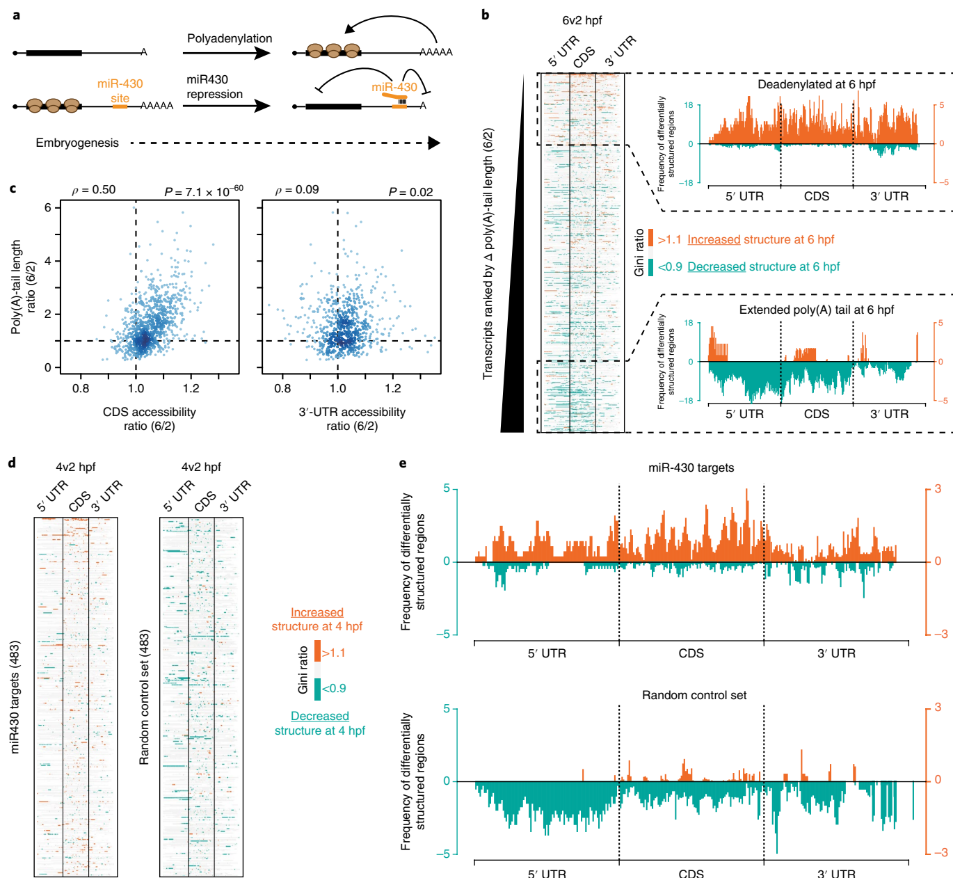
Fig. 4 | Polyadenylation and miR-430 activity influence mRNA structure. a , Schematic view of the effects of poly(A)-tail length and miRNA-mediated repression on translation during early embryogenesis. b , Left, structure changes along each transcript (total of 965 mRNAs with sufficient coverage in DMS-seq and poly(A)-tail-length profiling experiments at both 2 and 6 hpf), ranked by changes in poly(A)-tail length (6/2 hpf). Structure changes were identified by computation of the Gini ratio for each 100-nt sliding window (6/2 hpf). Right, cumulative distribution of differentially structured windows along the transcripts, for both the top 20% (top) and bottom 20% (bottom) transcripts, binned in poly(A)-tail length. c , Correlation between changes in poly(A)-tail length and accessibility (6/2 hpf), for both CDS (left; n = 939 ) and 3' UTR (right; n = 724 ). Spearman correlation coefficients ( \rho ) and the corresponding asymptotic P values are shown. d , mRNA structure changes along each of the miR-430 targets ( n = 483 ) or a random set of transcripts ( n = 483 ) taken from the non-miR-430 targets. Regions with structure changes were identified by computation of the Gini ratio for each 100-nt sliding window (4/2 hpf). e , Metaplot of the differentially structured regions along the transcripts, comparing 2 and 4 hpf (4v2), for both miR-430 targets ( n = 483 ) and non-miR-430 targets ( n = 1,495 ).
