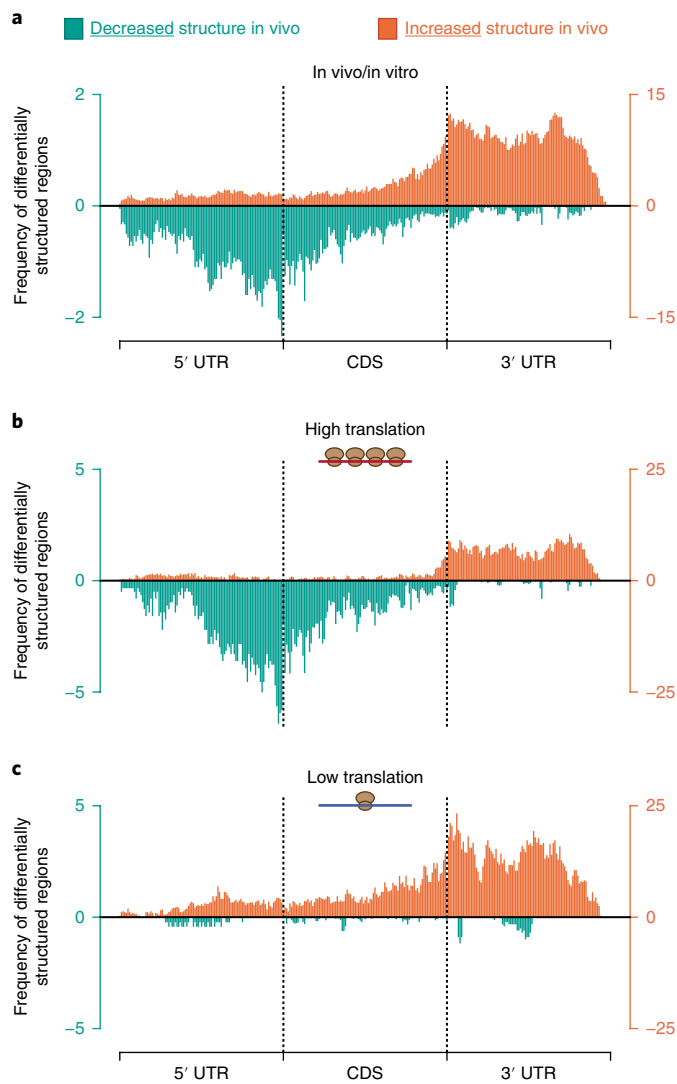
Fig. 5 | 3'-UTR regions are more structured in the cell than in vitro.
