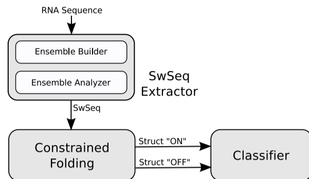
Fig. 1. Schematic view of the SwiSpot approach. Starting from an RNA sequence, a putative switching sequence is identified by the SwSeq Extractor. Such result is exploited by the Constrained Folding module to derive the two alternate structures. Finally, a classifier decides if a switching behavior can be associated to them.
