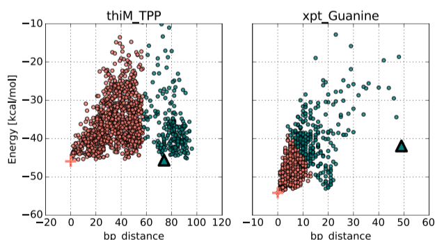
Fig. 3. Sampled and clustered structural ensembles for two different riboswitches. The two colours represent the clusters. The placement of ON/OFF conformations is indicated by the +/Δ symbols. In the right panel, the ensemble does not cover both of them (for sampled structural ensembles for the full reference dataset, see Figure S2).
